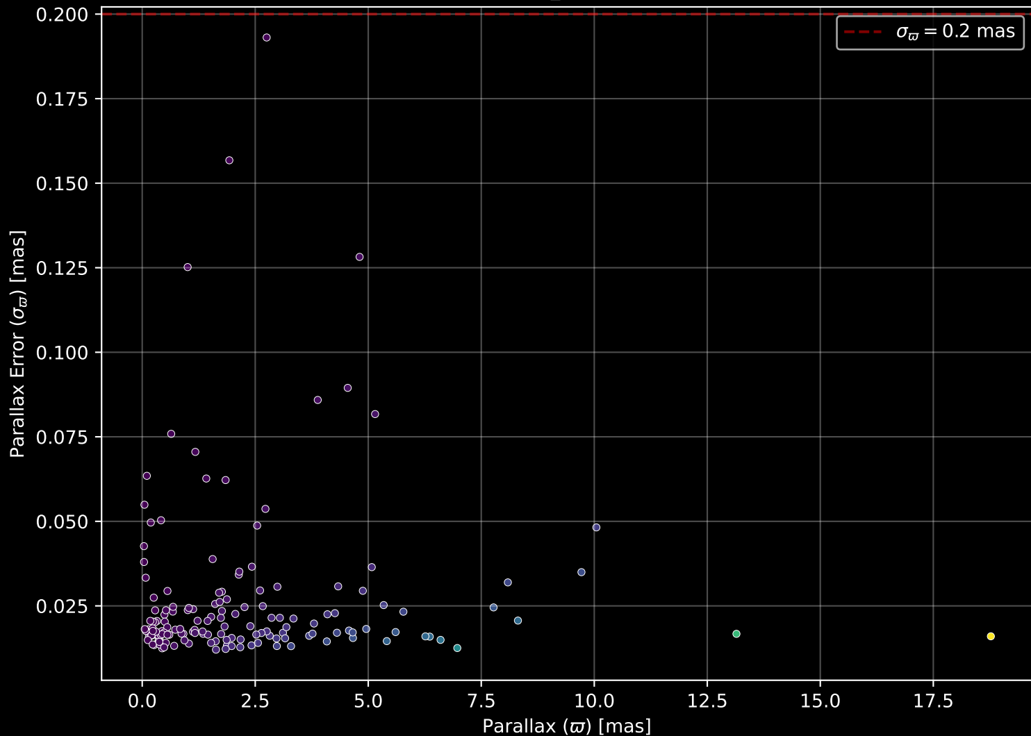
APOGEE DR17 Field: [040-27_MGA] Parallax Quality (n= 161)
