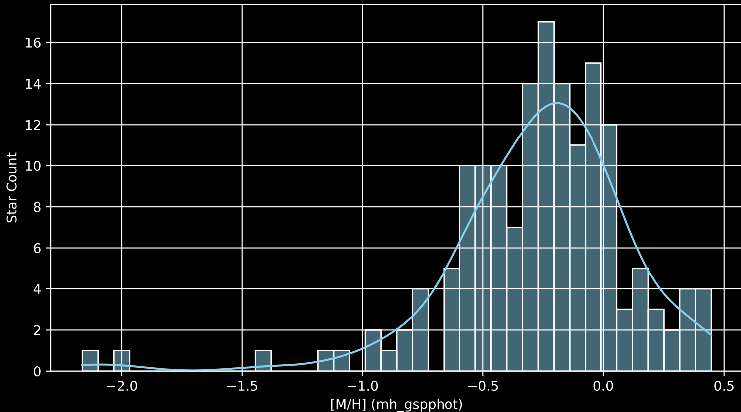
APOGEE DR17 Field: [040-27_MGA [M/H] (mh_gspphot) (n= 160)
