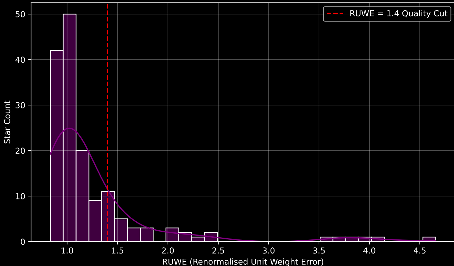
GAPOGEE DR17 Field [040-27_MGA] RUWE Distribution (n= 157)
