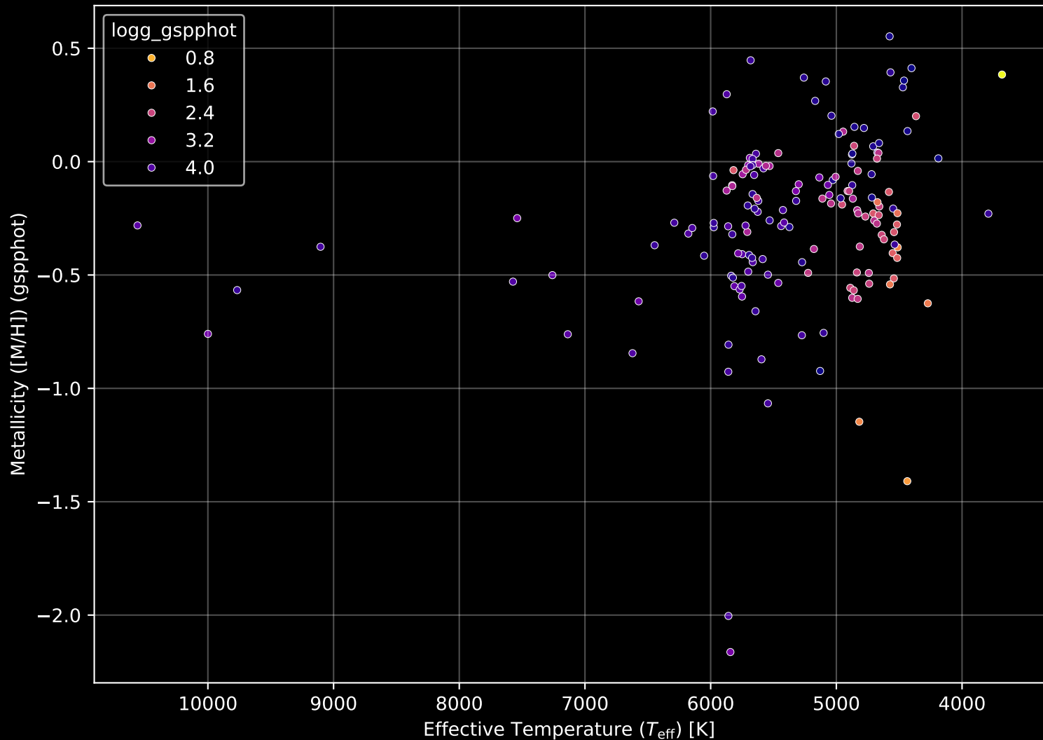
APOGEE DR17 Field: [040-27_MGA] Stellar Population Parameters (n= 161)
