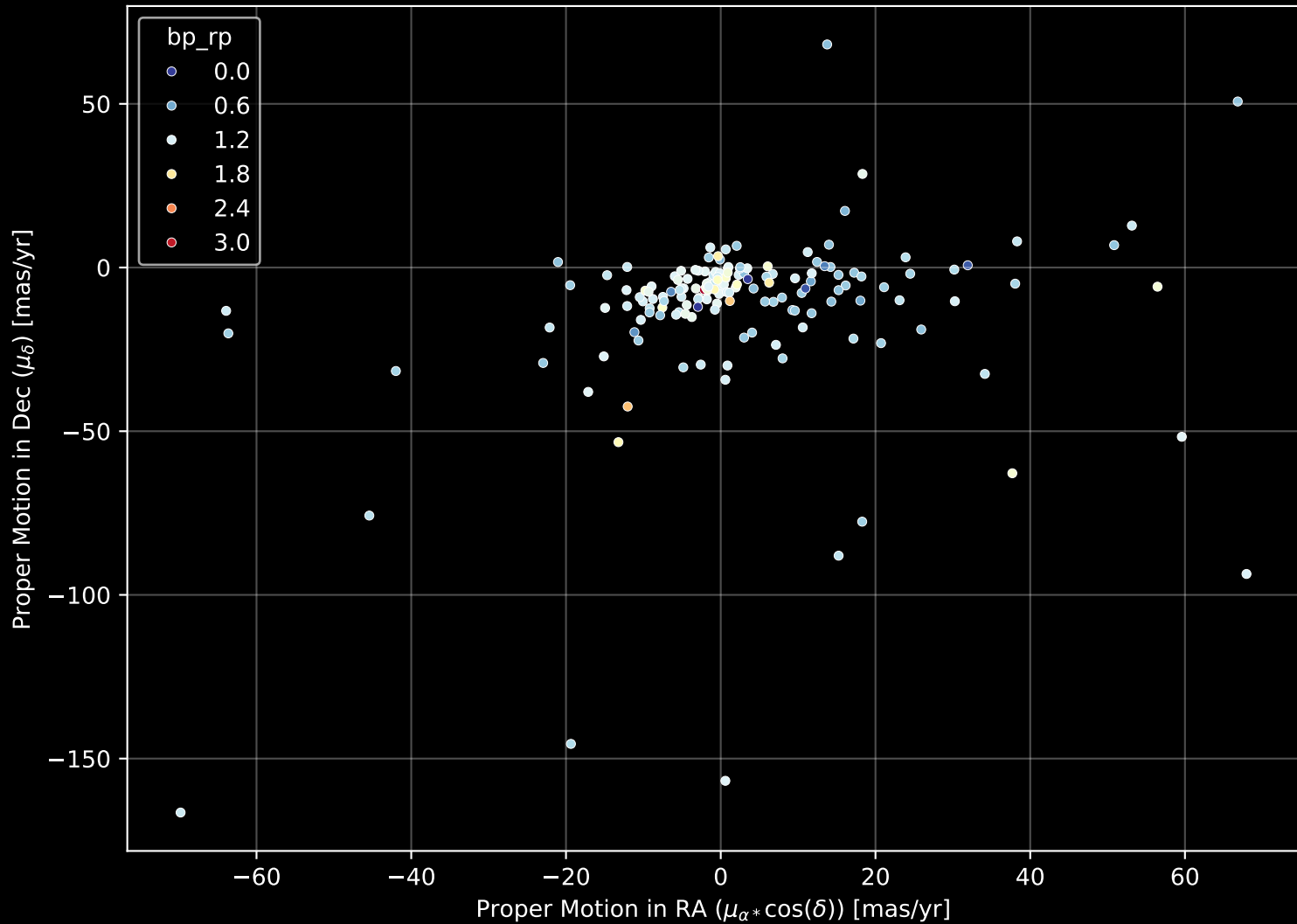
APOGEE DR17 Field: [040-27_MGA] Proper Motion Diagram (n= 161)
