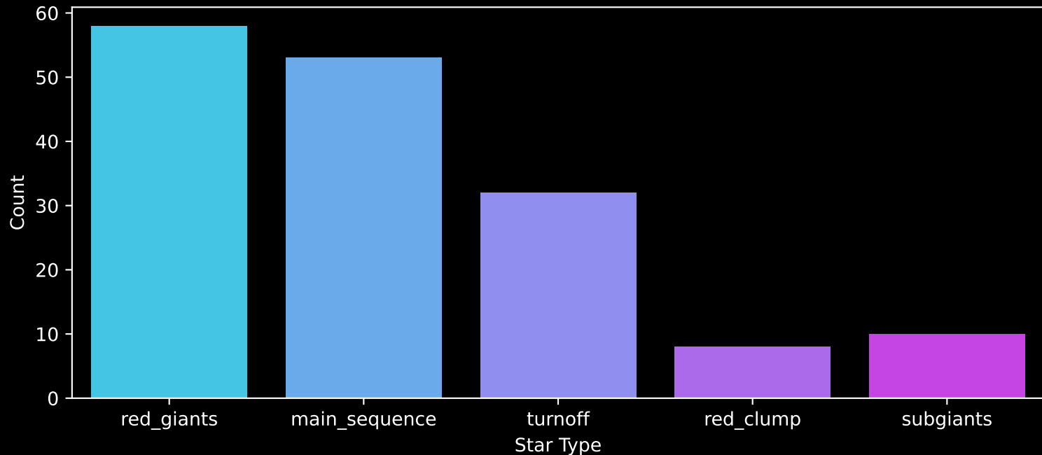
APOGEE DR17 Field: [040-27_MGA] Count plot of Star Type
