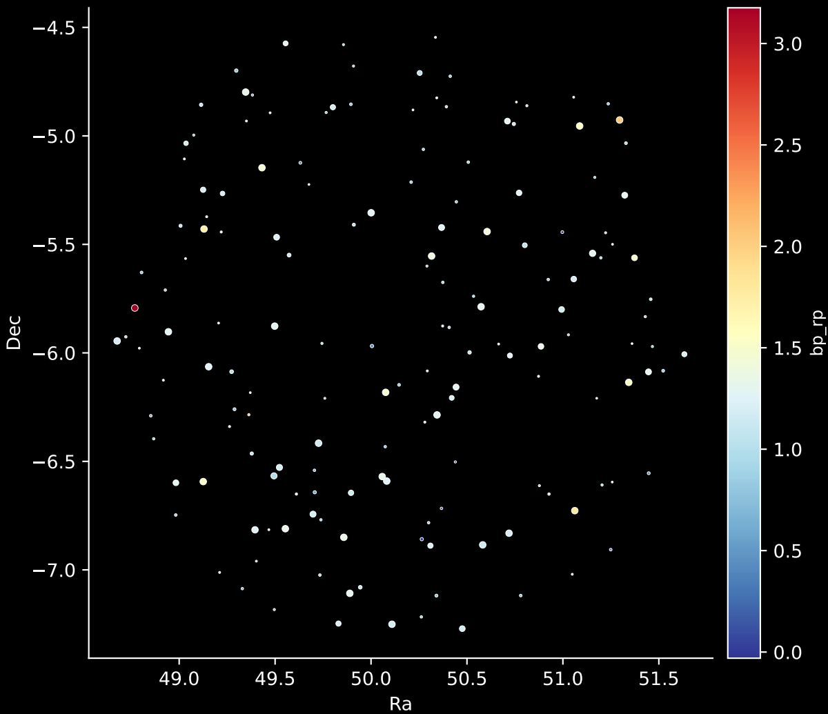
APOGEE DR17 Field: [040-27_MGA] Stars: 161
